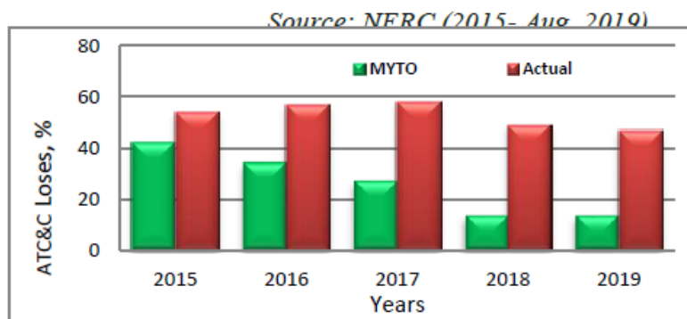
Figure 6: AT&C Loses, 2015-2019
